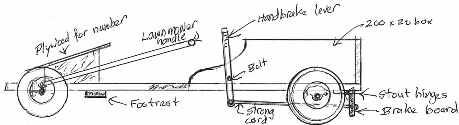
Diagram No. 1 Simple Box Trolley - Elevation - Plan
