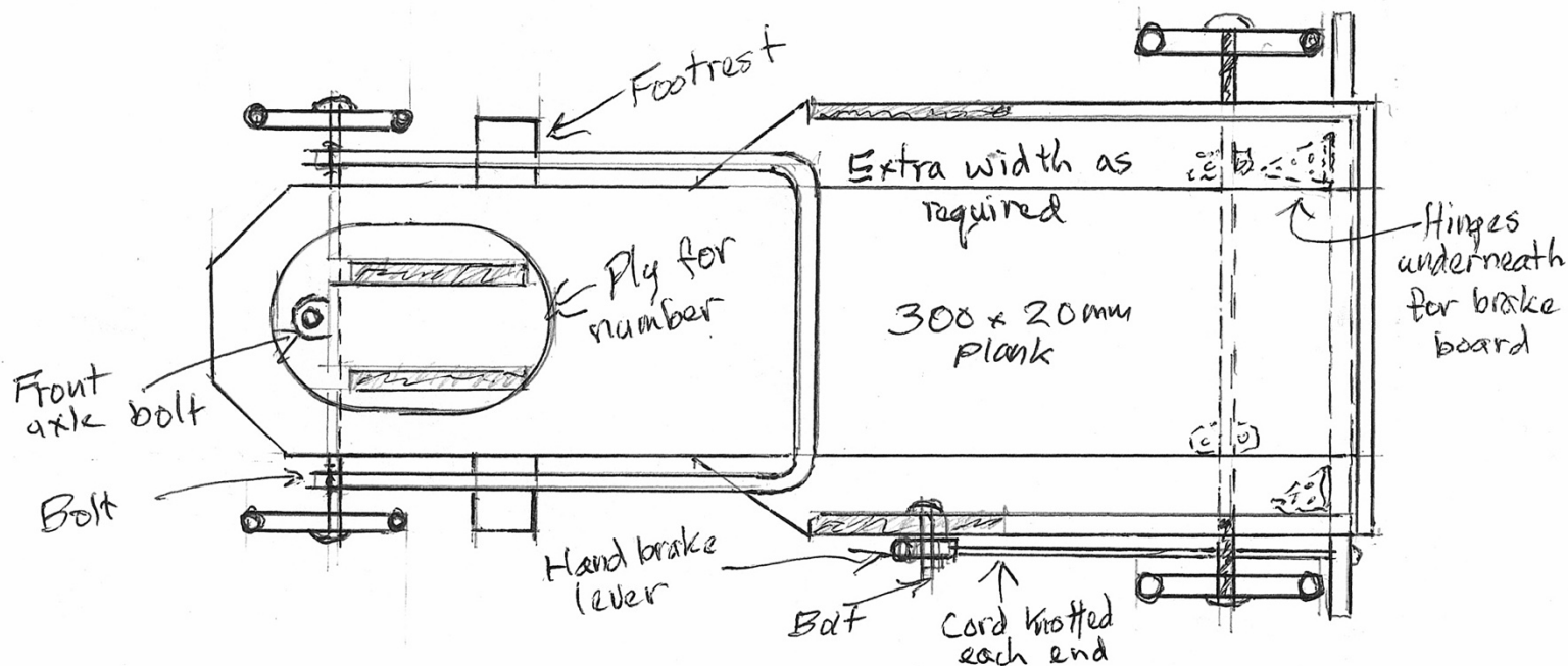
Diagram No. 1 Simple Box Trolley - Elevation - Plan
