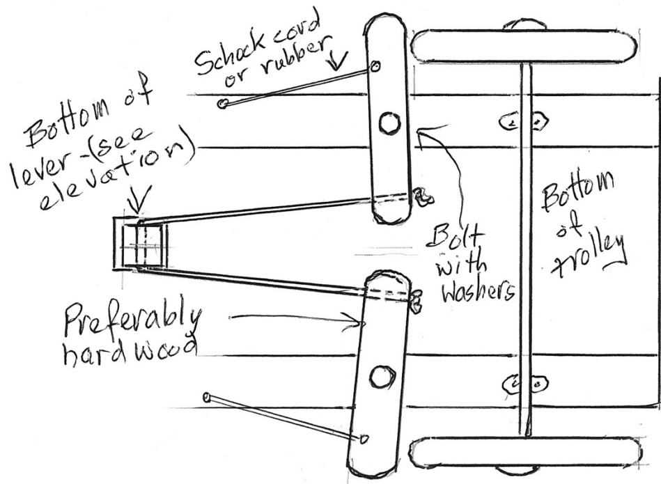
Alternative brake arrangement
